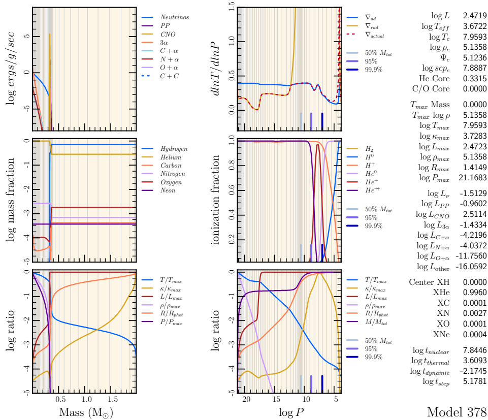
Figure 10: Profile 3
