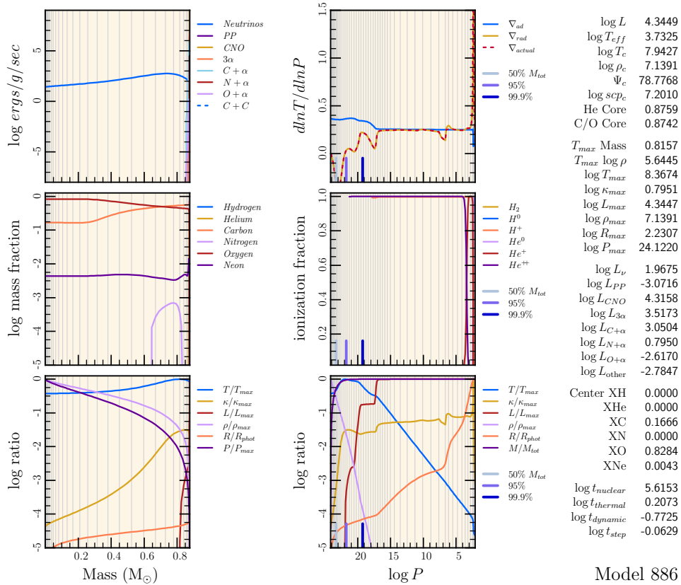
Figure 16: Profile 6
