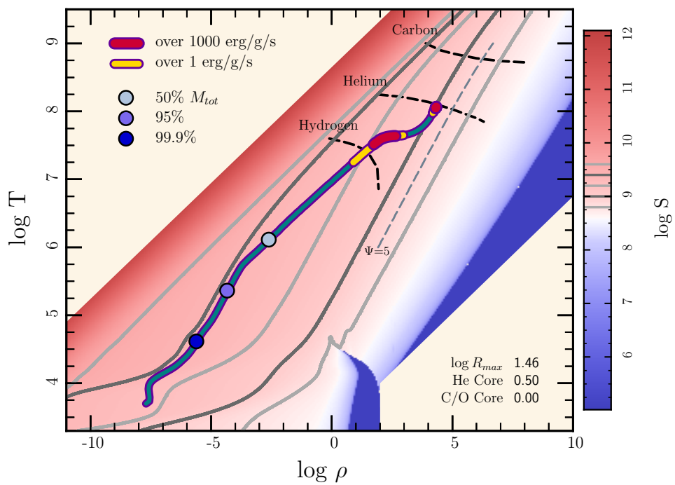
log S — Age 251.114 (Myr)
