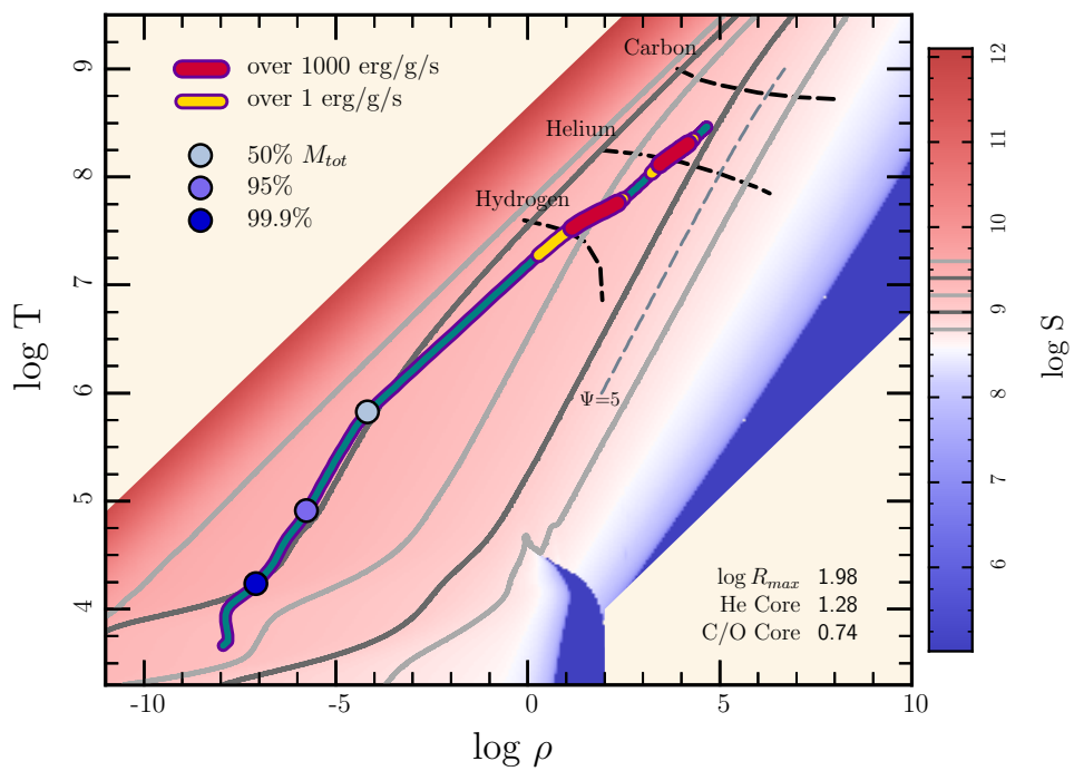
log S — Age 152.590 (Myr)
