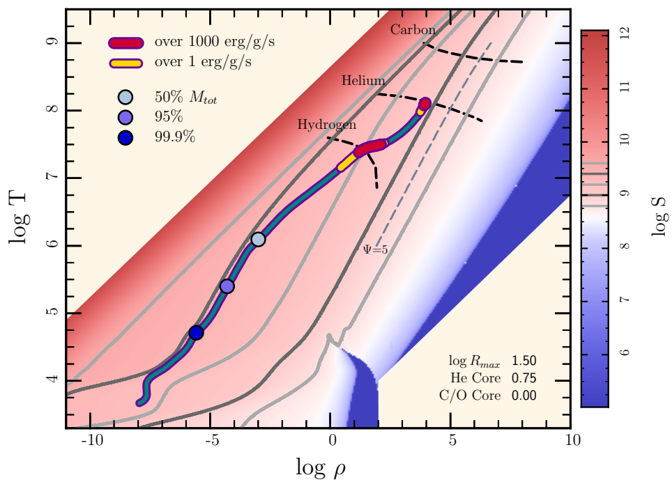
log S — Age 178.104 (Myr)
