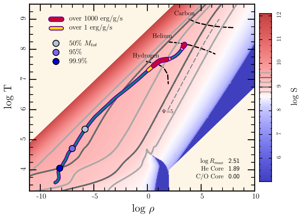
log S — Age 28.029 (Myr)
