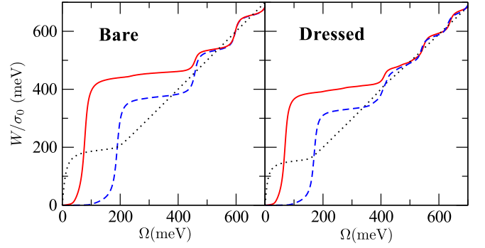
FIG. 12. (Color online) Partial optical sums for \mu_0 = 97\text{meV} (dashed blue curves) and \mu_0 = 230\text{meV} (solid red curves), with the same parameters as in Fig. 10. For comparison, the B = 0 case with \mu_0 = 97\text{meV} (dotted black curves) is also shown. Despite the splitting of levels in the dressed case, the optical weight follows the same pattern as in the bare case.
