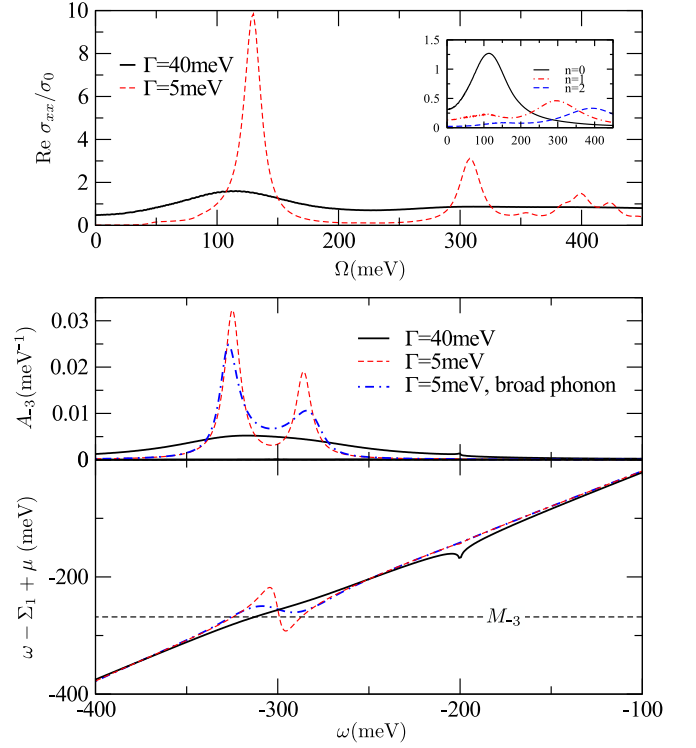
FIG. 19. (Color online) Effects of large broadening on the spectrum. The upper frame shows the diagonal conductivity for \Gamma = 40\text{meV} and 5\text{meV} ; the inset shows how the separate contributions to \text{Re } \sigma_{xx} overlap for the \Gamma = 40\text{meV} case. The lower two frames show a spectral function, A_{-3} , involving a split peak, along with the function \omega - \Sigma_1 + \mu that determines the nature of the peaks. Here results are shown for both a large impurity scattering and a broadened phonon; either effect, if sufficiently large, can annul the splitting of levels. In all cases, B = 18.2\text{T} , \mu_0 = 100\text{meV} , \omega_E = 200\text{meV} , A = 250\text{meV} . The broadened phonon distribution is a truncated Lorentzian with parameters A' = 555\text{meV} , \delta = 15\text{meV} , and \delta_0 = 30\text{meV} .
