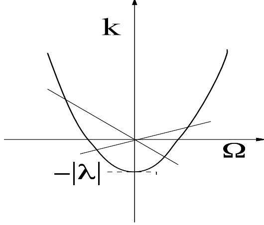
Figure 2: The dispersive curve (3.50) for negative \lambda . Any straight lines leaving the origin always intersect the curve.
