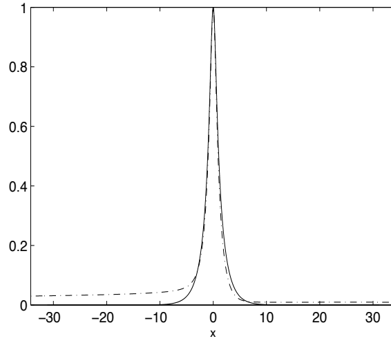
Figure 9: Initial (solid line) and final (dashed line) at t = 1.18 distributions for |\bar{\psi}| , interfacial waves, self-similar variables. The soliton amplitude was increased by 1%, \mu = 1 , \lambda = 1 . The ratio between final and initial soliton amplitudes in the physical variables is about 11.
