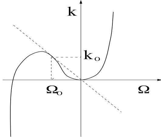
Figure 4: The third order dispersion k = D\Omega^2 + \gamma\Omega^3 . The straight line dispersive curve (3.50) for positive \lambda . The straight line (dashed) touches the dispersive curve at the point \Omega = \Omega_0 but intersects the curve at \Omega = 0 .
