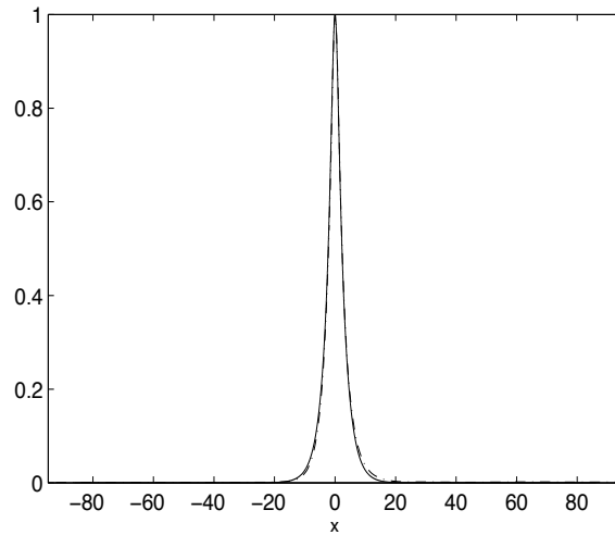
Figure 10: Initial (solid line) and final (dashed line) at t = 2.7192 distributions for |\bar{\psi}| , WW solitons, self-similar variables. The soliton amplitude was increased by 1%, \mu = 1 , \lambda = 1 . The ratio between final and initial soliton amplitudes in the physical variables is about 11.
