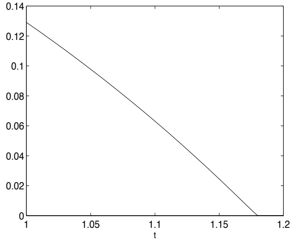
Figure 11: Dependence of 1/\max|\psi|^4 on time. Interfacial waves.
