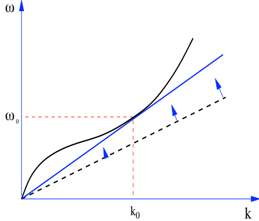
Figure 1: The solid line corresponds to the dispersion relation \omega = \sqrt{gk + \sigma k^3} for gravity-capillary waves. The dashed (straight) line corresponds to the soliton velocity. The arrows show the direction of increase of the soliton velocity. At the point \omega_0, k_0 , the straight line \omega = kV touches the dispersive curve.
