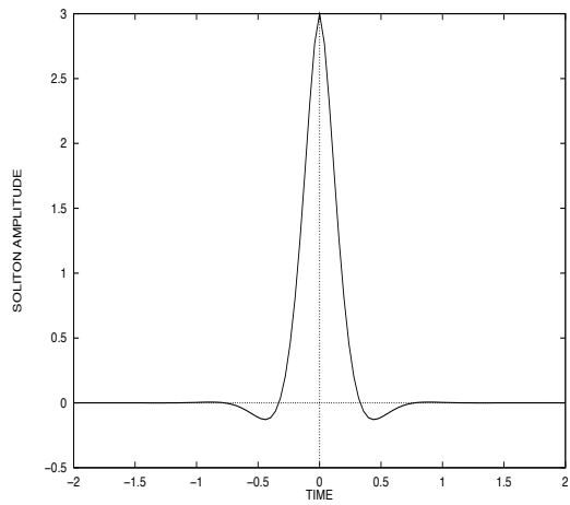
Figure 7: The soliton shape at \mu/\nu_0 = 10 . The oscillating tail is no longer visible.
