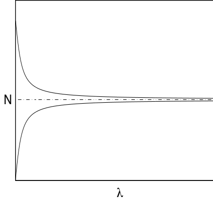
Figure 8: The dependence (5.14) of the number of particles N versus \lambda for two soliton families: \mu < 0 (lower curve) and \mu > 0 (upper curve)
