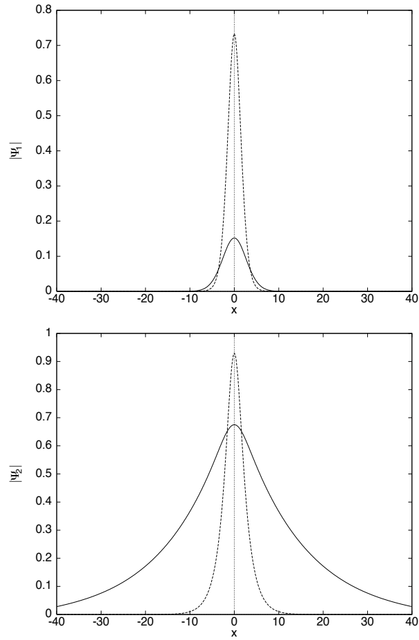
Figure 18: The functions |\psi_1(x)| and |\psi_2(x)| near the subcritical bifurcation boundary ( \Lambda_1^2 = \Lambda_2^2 + 1 and k = 1 ). Solid line is \Lambda_2 = 0.1 and the dashed line \Lambda_2 = 0.5 .
