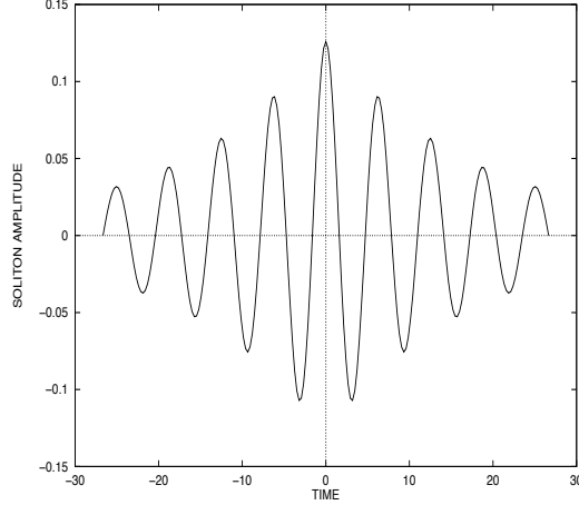
Figure 5: The soliton shape at \mu/\nu_0 = 1/3 . The soliton amplitude and time are measured in units \nu_0^2 and \nu_0^{-1} , respectively. The soliton envelope has a form which is close to the sech form.
