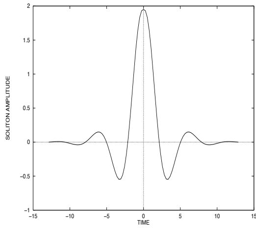
Figure 6: The soliton shape at \mu/\nu_0 = 1 . The soliton amplitude (in units \nu_0^2 ) grows and its duration (in units \nu_0^{-1} ) decreases. On the soliton size there are still some oscillations.
