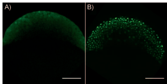
Figure 6. Induction of nuclear translocation of GFP-nls-ER T2 by photorelease of cyclofen-OH in wild-type zebrafish embryos injected with gfp-nls-ER T2 mRNA (100 ng \mu\text{L}^{-1} ) at the one-cell stage. Confocal GFP fluorescence image of embryos at 4 hpf (following incubation at 2 hpf for 90 min in 3 \mu\text{M} cInd and washing): A) without illumination, and B) 30 min after illumination with UV light; scale bar: 100 \mu\text{m} .
