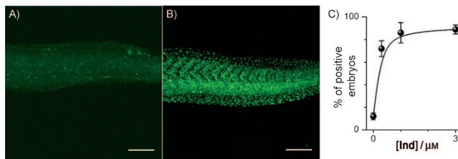
Figure 3. Induction of nuclear translocation of GFP-nls-ER T2 by addition of cyclofen-OH in wild-type zebrafish embryos injected with gfp-nls-ER T2 mRNA (100 ng \mu\text{L}^{-1} ) at the one-cell stage. GFP fluorescence image of embryos at 24–30 hpf after incubation with: A) 0, or B) 3 \mu\text{M} Ind . Note that the camera sensitivity was intensified by a factor of 6 in A) with respect to B). C) Dependence of the efficiency of nuclear translocation of GFP-nls-ER T2 on inducer concentration. Error bars are statistical errors estimated as \sqrt{p(1-p)/n} , where p is the percentage of embryos exhibiting a positive phenotype, and n is the total number of embryos investigated. The solid line is a guide for the eyes; scale bar: 100 \mu\text{m} .
