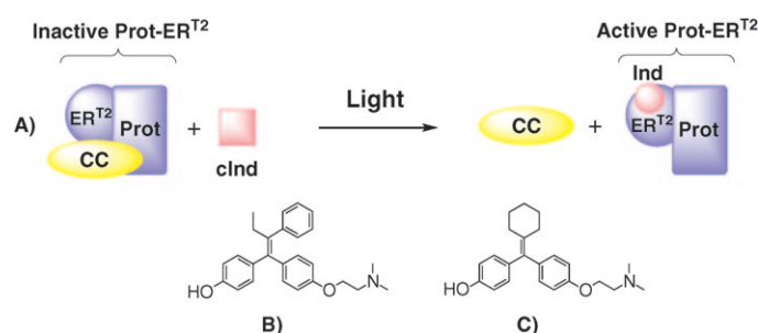
Scheme 1. A) The strategy to photoactivate properly engineered proteins. A protein fused to the ER T2 receptor (Prot; here a fluorescent protein linked to the receptor by a peptide acting as a nuclear localization signal) is inactivated by its assembly with a chaperone complex (CC). Upon photoactivation of a caged precursor (cInd), a nonendogenous inducer (Ind) is released and binds to the ER T2 moiety. The concomitant conformational change of the receptor causes assembly disruption and activates the ER T2 -fused protein. Examples of inducers: B) Ind: 4-hydroxy-tamoxifen (tamoxifen-OH), and C) 4-hydroxy-cyclofen (cyclofen-OH).
