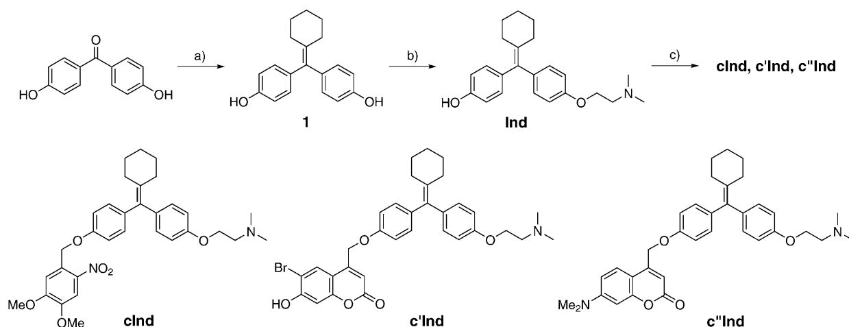
Scheme 2. Syntheses of 4-hydroxy-cyclofen ( Ind ) and its caged derivatives: a) cyclohexanone, \text{TiCl}_4 , Zn, THF, reflux, 2 h; b) \text{Cl}(\text{CH}_2)_2\text{N}(\text{CH}_3)_2\text{HCl} , \text{K}_2\text{CO}_3 , acetone/ \text{H}_2\text{O} , reflux, 18 h; c) caging alcohol, \text{P}(\text{Ph})_3 , diisopropyl azo dicarboxylate, THF, sonication, 20 min.
