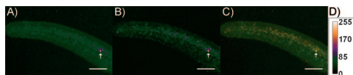
Figure 8. Images resulting from local photoactivation (750 nm, 10 mW, 10 s) of GFP-nls-ER T2 and mCherry-nls-ER T2 in the tail at 24 hpf in a wild-type embryo. A) GFP, and B) mCherry, and C) their superposition evidences the colocalization of these proteins after photoactivation; D) the images are intensity coded; scale bar: 100 \mu m.
