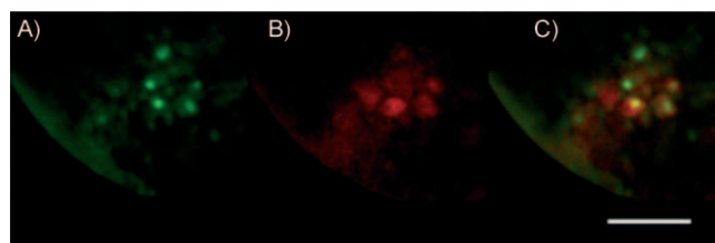
Figure 7. Images resulting from local photoactivation of GFP-nls-ER T2 in a wild-type embryo injected with gfp-nls-ER T2 mRNA and caged fluorescein dextran at the one-cell stage and conditioned as in Figure 6A and B. Emission from: A) GFP, B) fluorescein, and C) both fluorophores; scale bar: 100 \mu\text{m} .
