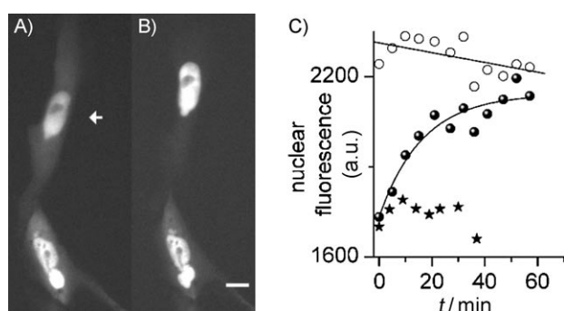
Figure 4. Selective nuclear GFP-nls-ER T2 translocation in one CV1 cell (indicated by an arrow in A) upon two-photon illumination (750 nm, 10 mW for 10 s). Fluorescence images of the targeted cell and a nearby unilluminated cell: A) 0, and B) 60 min after illumination. C) Time evolution of the mean nuclear fluorescence intensity in the targeted cell (●) and the reference cell (○) shown in A) and B). The stars depict the corresponding evolution for a cInd nonincubated control cells, which were illuminated similarly to the targeted cell in A). The CV1 cells were transfected with a gfp-nls-ER T2 plasmid, further incubated in 6 μM cInd for 30 min and washed before illumination; scale bar: 10 μm.
