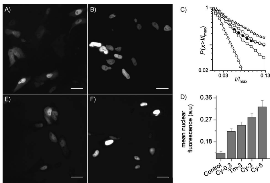
Figure 2. Induction of nuclear translocation of GFP-nls-ER T2 by addition or photorelease of cyclofen-OH in CV1 cells transfected with gfp-nls-ER T2 plasmid. GFP fluorescence image of CV1 cells 24 h after transfection and further incubation with: A) 0, or B) 3 \mu\text{M} Ind for 1 h (identical display range in A and B). C) Cumulative distribution after 0.0 ( \Delta ), 0.3 ( \square ), 3.0 ( \circ ) and 5.0 \mu\text{M} ( \star ) Ind , or 3.0 \mu\text{M} ( \bullet ) tamoxifen-OH treatment. D) Average value of the mean nuclear intensity; error bars represent standard errors of the mean. GFP fluorescence image of CV1 cells imaged 24 h after transfection and further incubation in 6 \mu\text{M} clnd for 30 min, E) without, and F) with global 365 nm UV illumination; scale bar: 10 \mu\text{m} .
