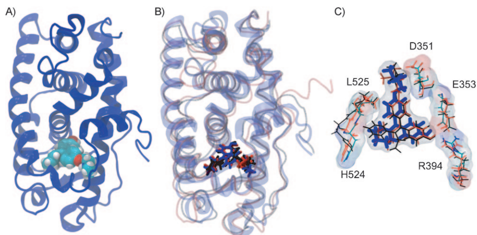
Figure 1. MD simulation snapshots. A) Representative structure of simulation C1 highlighting the position of the cyclofen-OH ligand within the ligand binding domain. The cyclofen-OH ligand remains solvent accessible through two accessibility sites: a large cleft, which could serve ligand binding and unbinding, and a channel that might enable solvent to hydrate the binding site; B) superposition of representative ligand binding domain-ligand complexes from simulations T1 (black), C1 (blue) and C2 (red). The actual values of the root mean square displacements (RMSD) of the protein stabilized beyond 20 ns are low, with C1 showing the least deviation (1.4 Å) and the reference simulation T1 was around 2 Å RMSD. The mutant C2 shows a slightly higher RMSD (2.9 Å) induced by the introduction of a longer side chain at position 351; C) zoom on the ligand binding site with key interacting residues (Arg394, Glu353, Asp351, His524, and Leu525).
