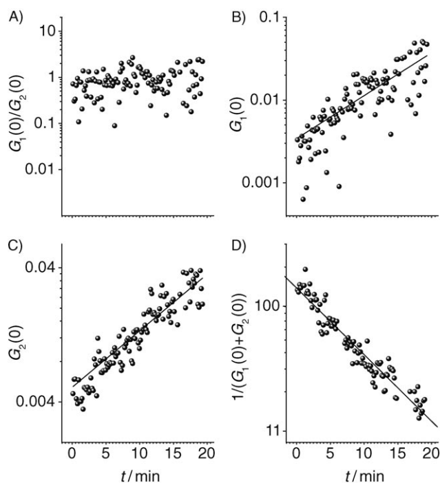
Figure 5. Analysis of the FCS autocorrelation curves of cytoplasmic GFP in a CV1 cell transfected with a gfp-nls-ER T2 plasmid, incubated in 6 \mu\text{M} cInd for 30 min and illuminated for 5 s with a UV laser (375 nm, 5 \mu\text{W} ; see also Figure S6 in the Supporting Information). Time dependence of: A) G_1(\tau=0,t)/G_2(\tau=0,t) , B) G_1(\tau=0,t) , C) G_2(\tau=0,t) , and D) 1/[G_1(\tau=0,t) + G_2(\tau=0,t)] extracted from a two-species model with \tau_1 = 1.7 ms and \tau_2 = 240 ms. Dots: experimental points; solid line: fit to an exponential decrease of the cytoplasmic species (due to nuclear translocation).
