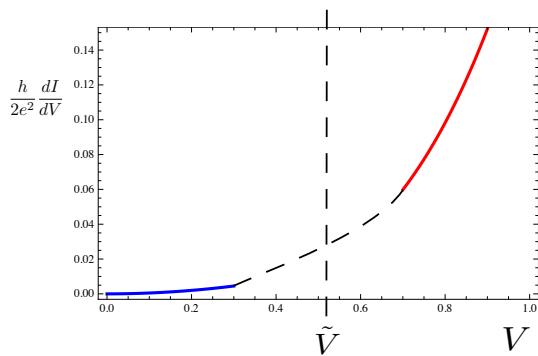
FIG. 6: Sample dI/dV curve as a function of voltage V (in arbitrary units) for g = 0.7 in a helical nanowire/non-topological superconductor junction. The red portion is calculated according to Eq. (95), while at sufficiently low voltages (blue curve) the Fermi liquid leads dominate and we have a crossover to g = 1 scaling.
