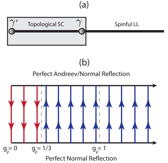
FIG. 4: (a) Topological superconductor forming a junction with a spinful Luttinger liquid. (b) Flow diagram for the junction as a function of the charge-sector interaction parameter g_\rho for the Luttinger liquid when the spin-sector interaction parameter is g_\sigma = 1 . For g_\rho < 1/3 the system flows to a perfect normal reflection fixed point characterized by a vanishing zero-bias conductance. When g_\rho > 1/3 , however, the junction flows to a novel fixed point corresponding to perfect Andreev reflection for one species and perfect normal reflection for the other, yielding a quantized 2e^2/h conductance.
