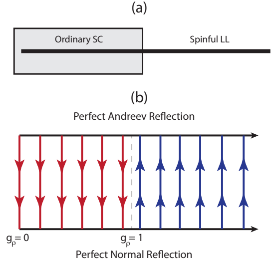
FIG. 3: (a) Trivial superconductor forming a junction with a spinful Luttinger liquid. (b) Flow diagram for the junction as a function of the charge-sector interaction parameter g_\rho for the Luttinger liquid, in the limit where the spin-sector interaction parameter is g_\sigma = 1 . Note that the free-fermion limit is very special—here there are marginal boundary couplings which lead to a non-universal zero-bias conductance ranging anywhere from 0 to 4e^2/h depending on parameters. For any repulsive interaction strength ( g_\rho < 1 ), however, the junction flows to the perfect normal reflection fixed point where the zero-bias conductance vanishes.
