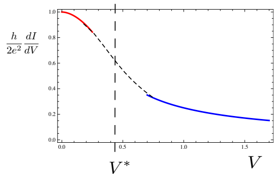
FIG. 5: Sample dI/dV curve as a function of voltage V (in arbitrary units) for g = 0.95 in a helical nanowire/topological superconductor junction. The blue and red portions are the perturbative results around the normal and Andreev fixed points respectively, calculated according to Eq. (91).
