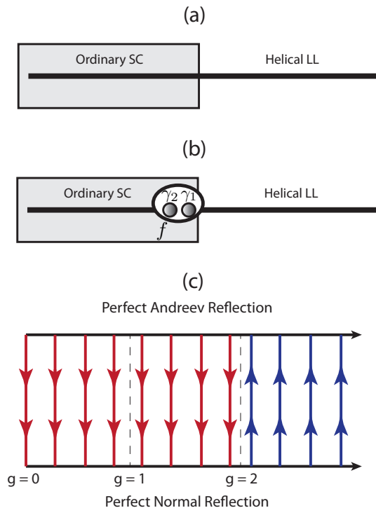
FIG. 2: (a) Ordinary superconductor forming a junction with a helical Luttinger liquid. If the superconductor is fully gapped throughout, then in the non-interacting limit the helical wire necessarily flows to a fixed point at which perfect normal reflection occurs at the junction. Accessing the perfect Andreev reflection fixed point in the non-interacting limit requires the presence of a zero-energy Andreev bound state f = (\gamma_1 + i\gamma_2)/2 at the junction as shown schematically in (b), with fine-tuning such that the wire couples only to (say) \gamma_1 . (c) Flow diagram for the junction as a function of the interaction parameter g for the Luttinger liquid. For helical Luttinger liquids with g < 2 , the perfect normal reflection fixed point is stable. When g > 2 , however, this fixed point is unstable towards the Andreev fixed point. Remarkably, here the Andreev bound state required to achieve perfect Andreev reflection will be generated dynamically, and with no fine-tuning required.
