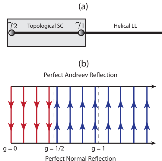
FIG. 1: (a) Topological superconductor forming a junction with a helical Luttinger liquid. We assume that the helical Luttinger liquid couples only to the Majorana \gamma_1 at the interface, while its partner \gamma_2 remains a robust zero-energy mode. (b) Flow diagram for the junction as a function of the interaction parameter g for the Luttinger liquid. Provided g > 1/2 , coupling to the Majorana \gamma_1 causes the Luttinger liquid to flow onto a fixed point where perfect Andreev reflection occurs at the junction. Here the zero-bias conductance for the junction is quantized at 2e^2/h . For Luttinger liquids with strong repulsive interactions such that g < 1/2 , however, coupling to \gamma_1 is irrelevant. Here the system flows onto a fixed point where the Luttinger liquid undergoes perfect normal reflection at the junction, leading to a vanishing zero-bias conductance.
