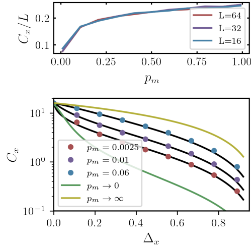
Figure 13: Steady state coherence C_x as a function of p_m and \Delta_x = (p_x - p_z) for p_y = p_R = p_e = 0 . The top figure shows volume-law coherence C_x for \Delta_x = 0.5 obtained via Clifford simulations. It shows no evidence of a phase with area-law coherence for finite p_m . The bottom figure shows the steady state coherence C_x for different values of p_m and a system size L = 32 . The colored dots are data computed via Clifford simulations, while the solid lines correspond to the predictions using the coherence rate equations derived in the text. The three black lines correspond to the rate equation Eq. 12 where the lengths scales \xi = (2.7, 5, 8) are found by best fit for the Clifford simulation data at p_m = (0.06, 0.01, 0.0025) respectively.
