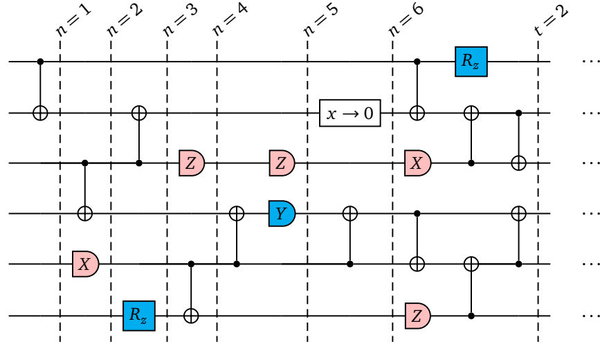
Figure 3: An example of the random hybrid circuit studied in the text. Each gate has an effect on the coherence in either the X or Z basis: preserves coherence in both basis (white), generates coherence in X basis (blue), or destroys coherence in either X or Z basis (red). At each step n , a CNOT gate is applied to two neighboring qubits with probability p_u = 1 , a measurement in the X , Y and Z basis is performed at a random site with probabilities p_m p_x, p_m p_y and p_m p_z respectively, a phase gate R_z is applied with probability p_R , and a bit eraser error occurs with probability p_e . Time is measured as t = n/L and since a CNOT is performed at each time step ( p_u = 1 ), the circuit above shows t = 2 after 12 = 2L random CNOTs have occurred.
