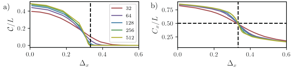
Figure 10: a) This figure shows the quantum channel capacity \mathcal{C} , computed by the purification dynamics, at a time t = 5L , for the same circuits studied in Fig. 9. It shows a transition at \Delta_x \approx 1/3 (marked by a black vertical dashed line), the location of the critical point determined by the competition of coherence generating and coherence destroying measurements p_y > |p_x - p_z| . b) Coherence for the same circuit but with an initial pure state. The coherence crosses C_x = L/2 at the critical point \Delta_x = 1/3 as predicted by the rate Eq. 12.
