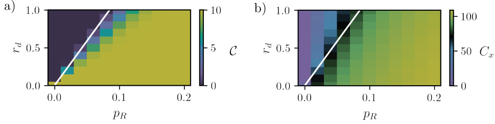
Figure 11: Quantum channel capacity \mathcal{C} for a diary encoding |A| = 10 qubits (panel a) and X basis coherence C_x (panel b) at time t = 10 for a circuit composed of CNOTs, single bit phase gates occurring at a rate p_R , and two types of attack operations occurring at a rate p_m + p_e = 0.05 : X measurements occur at a rate p_m = 0.05 * r_d (i.e. p_x = 1 and p_y = p_z = 0 ) while coherence-maintaining bit erasers occur at a rate p_e = 0.05(1 - r_d) . Panel a) demonstrates a transition between zero and finite quantum channel capacity for sufficiently large rate of coherence generating phase gates. Panel b) shows that this transition is associated with a sharp change in coherence C_x . The color scheme in the panel b) is chosen such that C_x = L/2 = 64 is black.
