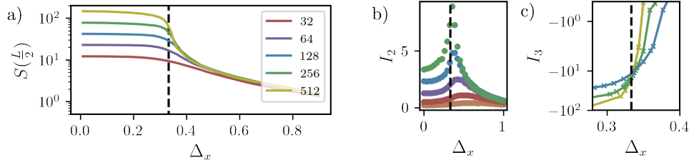
Figure 9: a) Half cut entanglement entropy S(L/2) v.s. imbalance between X and Z measurements \Delta_x = (p_x - p_z)/(1 - p_y) . The \Delta_x = 1/3 critical point predicted by p_y = |p_x - p_z| is confirmed by the b) Anti-podal mutual information I_2 and b) tripartite mutual info I_3 as discussed in the text. Different lines correspond to the system sizes shown in the legend. In this figure p_m = 0.01 , p_y = 1/4 and p_R = p_e = 0 .
