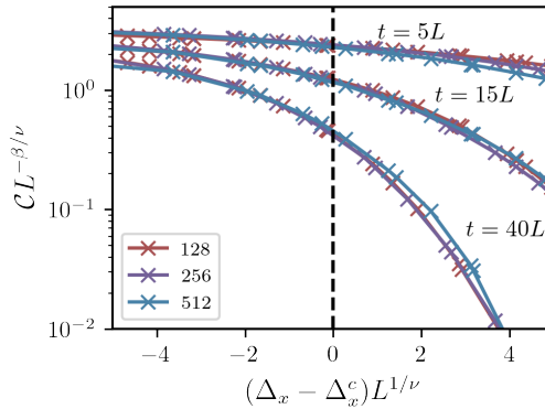
Figure 15: Scaling collapse for the coherent information, \mathcal{C} , occurring at three different times t = 5L, 15L and t/L = 40 as labeled in the figure. In this figure \Delta_x^c = 0.33 \pm 0.02 , \nu = 1.09 \pm 0.05 and \beta = 0.65 \pm 0.05 , where the variation in the exponents arises from both sampling error as in Fig. 14 and from variations in the best fit critical parameters at the three different times. The length critical exponent, \nu is compatible by a single standard deviation with the one obtained in Fig. 14 for the tripartite mutual information.
