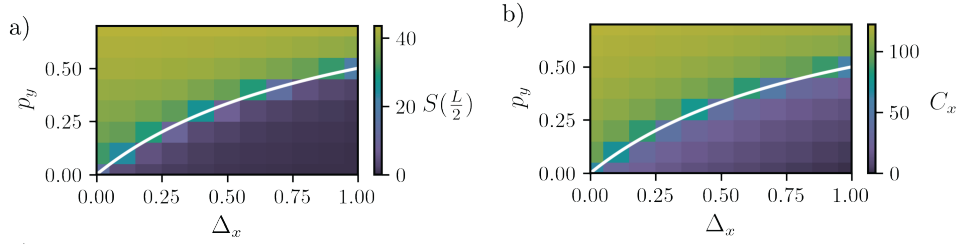
Figure 8: (a) Steady state half cut entanglement, S(x = L/2) , and (b) coherence, C_x , for the hybrid circuits with a sequence of random CNOTs and X , Y and Z measurements for the small measurement rate of p_m = 0.01 ( p_R = 0 and p_e = 0 ). In these figures \Delta_x parameterizes the imbalance between X and Z measurements \Delta_x = (p_x - p_z)/(1 - p_y) . These figures show the critical line (white), |\Delta_x| = p_y/(1 - p_y) , which is predicted by the competition between coherence loss and growth rates as discussed in the text. Due to the duality between the X and Z bases, dynamics are the same for \Delta_x \rightarrow -\Delta_x . For the \Delta_x > 0 side of the duality, the coherence in the Z basis, C_z , is greater than C_x and does not constrain the entanglement. These figures were computed with L = 128 and averaging over 2000 circuit realizations.
