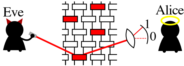
Figure 1: Cartoon hybrid circuit composed of unitaries (white) and measurements (red), which can be viewed as an information game played between Alice and Eve. In this game, Alice attempts to store her diary in a set of qubits and Eve attempts to destroy her diary by measuring them (for instance, shining light on the qubits). To protect her diary, Alice applies a set of unitaries in an attempt to protect her diary from Eve’s measurements, which Eve can apply at a fixed rate relative to the rate at which Alice can apply unitaries. Alice is allowed to capture the emitted light, record the measurement outcomes, and knows the measurement basis Eve makes a measurement in. In this way, Alice can keep track of the evolving state of the system, such that she might be able to apply a unitary at the end of the game to recover her diary. The measurement-induced phase transition occurs when random strategies are played, and corresponds to a transition in the quantum channel capacity between the initial state encoding Alice’s diary, and the final state at the end of the game. Alice wins the game in the volume-law phase when the quantum channel capacity is finite, while she loses the game in the area-law phase when the channel capacity is zero.
