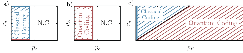
Figure 12: Alice’s coding capabilities in various regions of parameter space with p_z = p_y = 0 and p_x = 1 . In all figures, we consider Eve’s attacks to be coherence-maintaining bit erasers (at a rate p_e ) and X measurements (at a rate p_m = p_e r_d / (1 - r_d) ), and we give Alice the option to apply phase gates up to a rate p_R . a) For p_R = 0 , Alice can only encode a quantum diary if Eve does not apply coherence destroying measurements (red line at r_d = 0 ), otherwise Alice can protect a classical diary as long as p_e is sufficiently small. b) In this figure p_m = 0 and so Alice can always protect a quantum diary as long as she can protect a classical diary. When p_R = 0 , we retrieve the limit discussed in section 3.2 where only coherence-maintaining bit erasers are applied. c) In this figure p_e = 0.05 - p_m as in Fig. 11, but now Alice has the choice to apply phase gates or not. The figure shows the transition to quantum error correction as in Fig. 11, but now if she chooses not to apply phase gates she can protect classical information so long as p_e < 0.1 .
