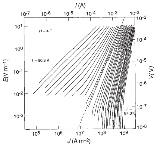
FIG. 5 Current-voltage ( I - V ) curves at fixed temperatures for a 0.4- \mu\text{m} -thick YBCO epitaxial film in a 4-T magnetic field applied parallel to the material's c -axis. Adjacent curves differ by temperature intervals of \sim 0.3 K, with the highest and lowest temperatures as indicated. The curves are on logarithmic scales, and the current densities J and electric fields E are also indicated. The dashed line indicates the vortex-glass transition temperature at T_{\text{vg}} \approx 77 K at which E \sim J^{(z+1)/2} with z \approx 4.8 \pm 0.2 . For temperatures above T_{\text{vg}} at low current densities, E \sim J , indicating the ohmic behaviour characteristic of a normal metal or vortex fluid. Below T_{\text{vg}} , the slope of the curves becomes steeper and steeper at low voltages suggesting exponentially small dissipation as predicted for the vortex-glass phase. Data are from ref. 20. The curves were measured in separate sweeps up to E \approx 1 \text{ V m}^{-1} and to E \approx 10 \text{ V m}^{-1} . The breaks between the two sets of curves at E \approx 1 \text{ V m}^{-1} are due to resistive heating in the larger E sweeps.
