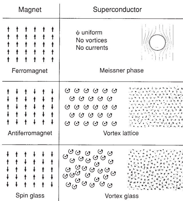
FIG. 2 Patterns of spin order in magnetically ordered systems (left, where arrows indicate the orientation of the local spins) and the analogous ordered phases of a superconductor (right). In the Meissner phase of the superconductor (top) the magnetic field and the vortices are expelled from the material, as indicated by the magnetic field lines around an ideal spherical superconducting ball. For the vortex lattice and glass, the positions of the vortex cores are indicated by dots and the circulating currents by arrows in the schematic drawings; on the right are images of vortex patterns on BSCCO crystals obtained by decorating the surface with fine magnetic particles that preferentially stick near the magnetic flux lines on each vortex. The decoration images are from the work reported in ref. 36.
